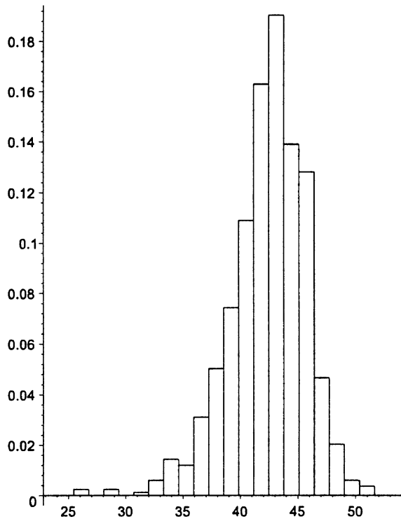
Fig. 1. Histogram of the thickness of razor heads for the first sample of 835 measurements.
