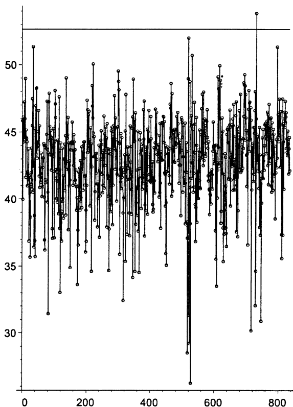
Fig. 2. Control chart of the second sample of 835 measurements of the thickness of razor heads.
