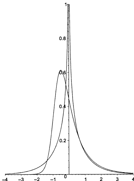
Fig. 3. Density of the normal inverse Gaussian (2,1.5) and the corresponding density of the normal power family with \gamma = 0.77 .
