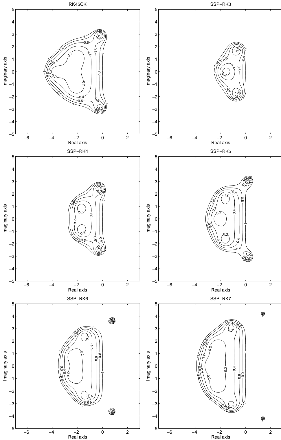
Figure 2: Stability regions for the five-stage fourth-order Runge-Kutta method (top left) and for five different SSP-RK methods of order m = 3, 4, 5, 6, 7
