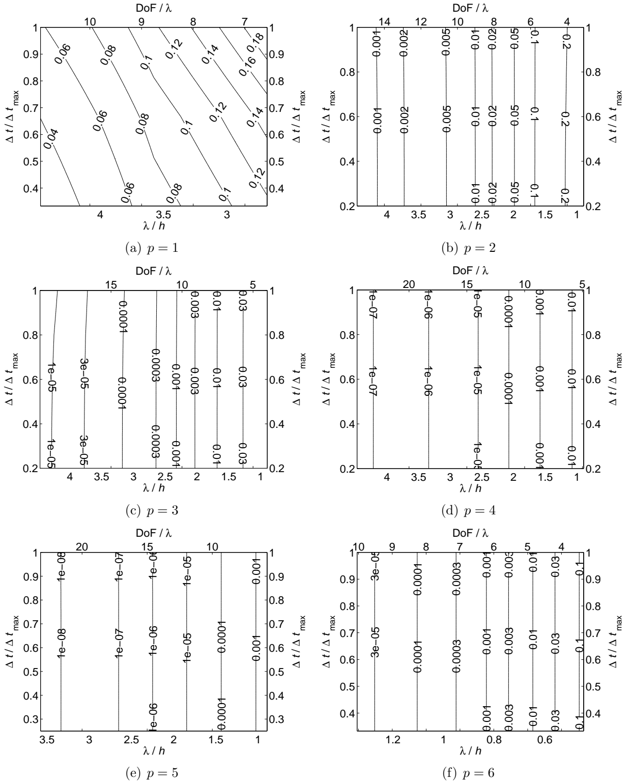
Figure 5: Absolute value the of dispersion error as a function of wave length per mesh size ( \lambda/h ), degrees of freedom per wavelength ( \text{DoF}/\lambda ) and relative time step ( \Delta t/\Delta t_{\max} ) for polynomial orders p = 1, 2, 3, 4, 5, 6 on a uniform mesh
