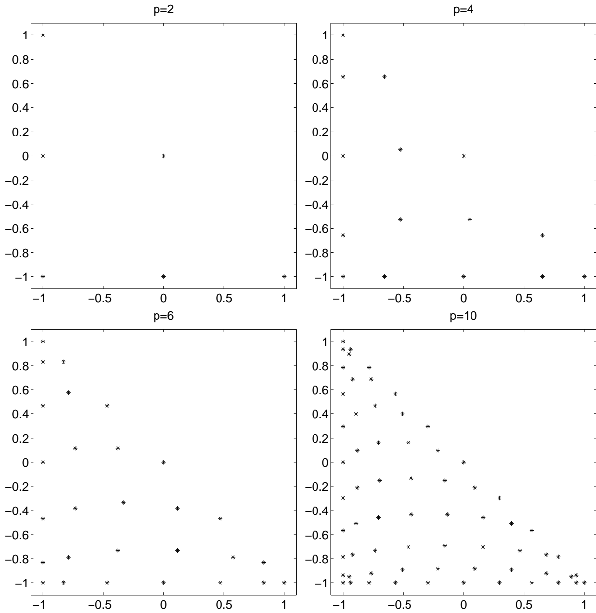
Figure 1: Electrostatic points for orders p = 2, 4, 6, 10
