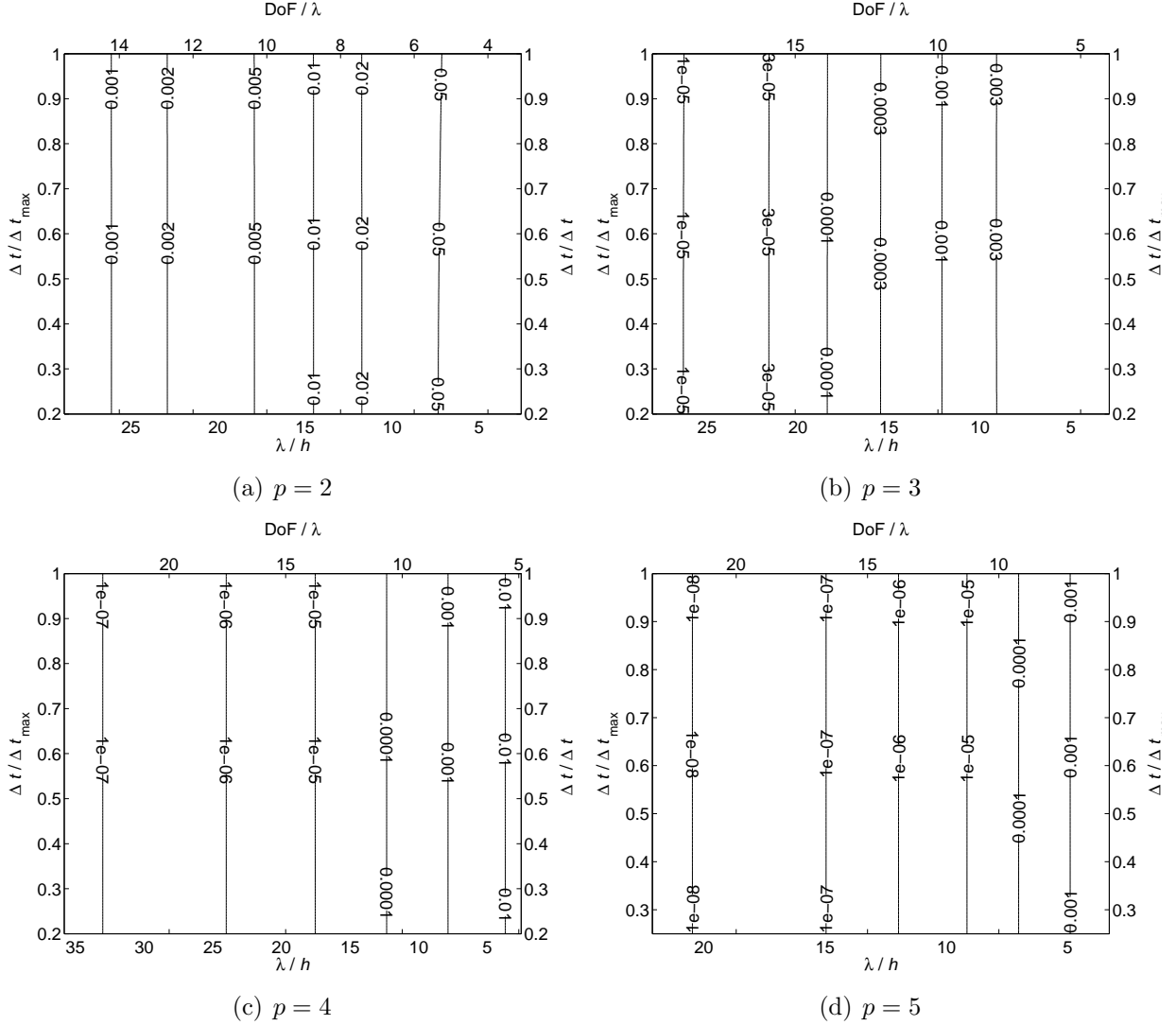
Figure 7: Absolute value of the dispersion error as a function of wave length per mesh size ( \lambda/h ), degrees of freedom per wavelength ( \text{DoF}/\lambda ) and relative time step ( \Delta t/\Delta t_{\max} ) for polynomial orders p = 2, 3, 4, 5 on a non-uniform random mesh
