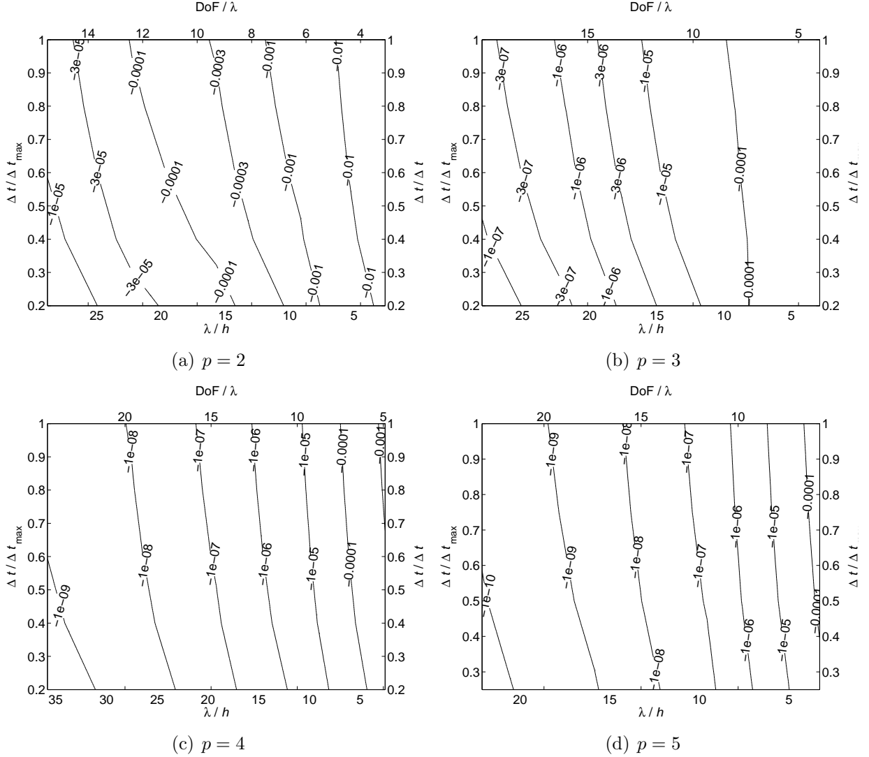
Figure 8: Dissipation error as a function of wave length per mesh size ( \lambda/h ), degrees of freedom per wavelength ( \text{DoF}/\lambda ) and relative time step ( \Delta t/\Delta t_{\max} ) for polynomial orders p = 2, 3, 4, 5 on a non-uniform random mesh
