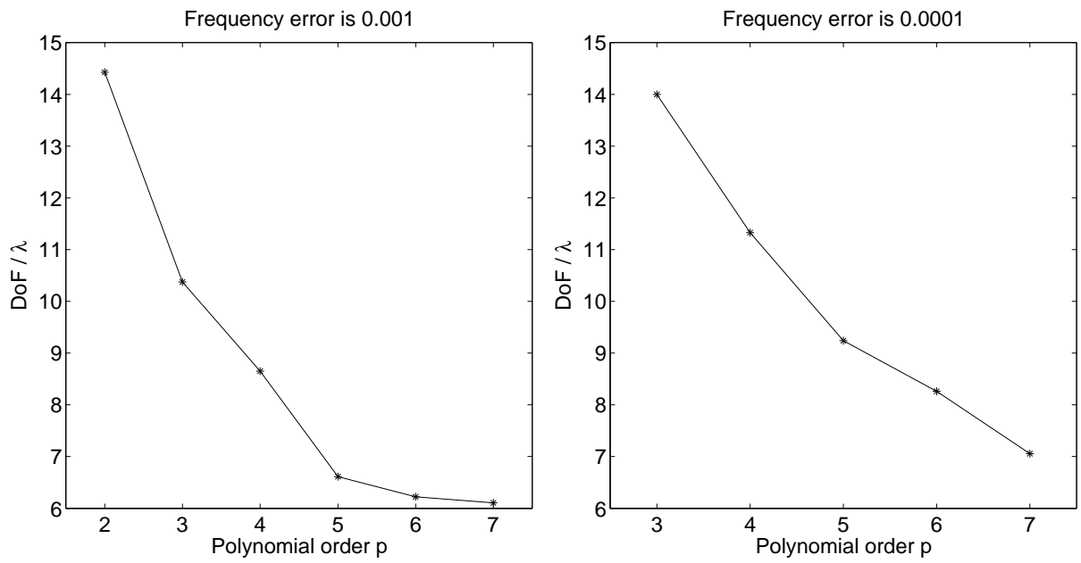
Figure 9: Degrees of freedom as a function of polynomial order for given dispersion error 10^{-3} and 10^{-4} on uniform meshes
