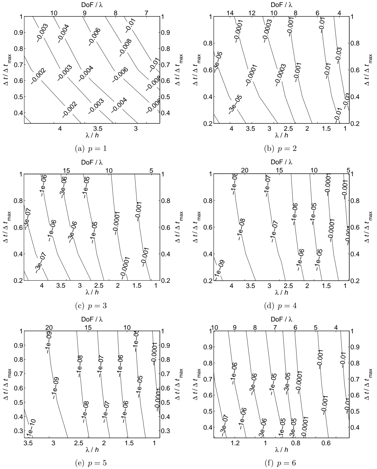
Figure 6: Dissipation error as a function of wave length per mesh size ( \lambda/h ), degrees of freedom per wavelength ( \text{DoF}/\lambda ) and relative time step ( \Delta t/\Delta t_{\max} ) for polynomial orders p = 1, 2, 3, 4, 5, 6 on a uniform mesh
